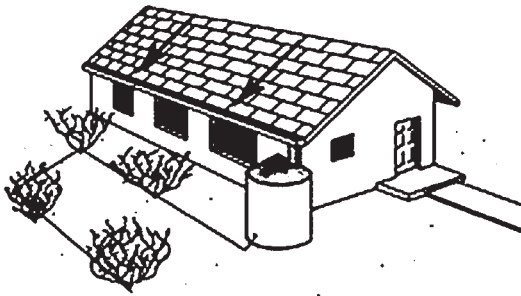
Water harvesting system with roof catchment, gutter, downspout, storage and drip distribution system. Source: Arizona Department of Water Resources. ©1998
